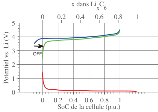
(c) LR = 110 \% , OFF = 10 \%
